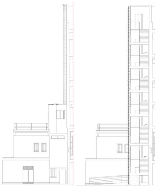
CROSS SECTION OF THE NEW VERTICAL CONNECTION: ANTE OPERAM AND POST OPERAM
