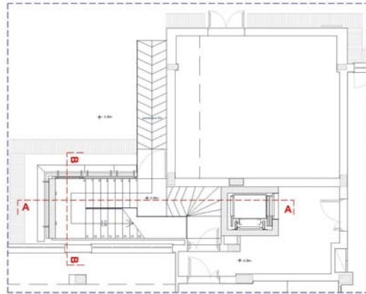
PLAN OF THE NEW VERTICAL CONNECTION IN THE BASEMENT
