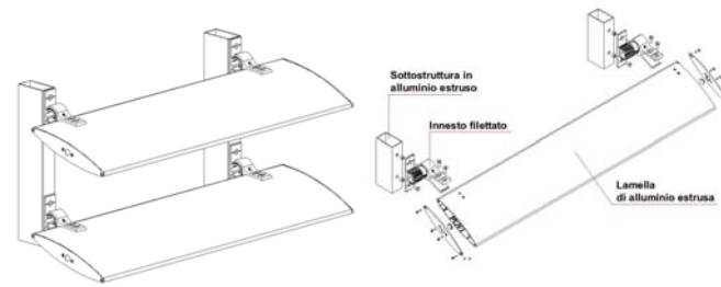
SUNBREAKERS PARTICULARS
