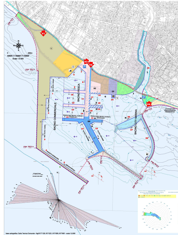
MASTER PLAN
