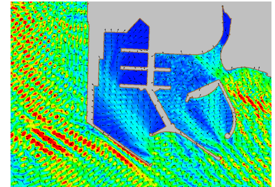
HYDRAULIC-MARITIME STUDIES
