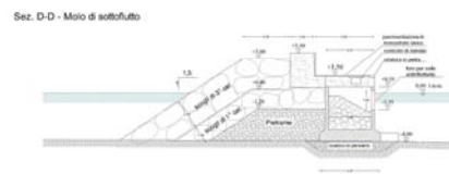
TYPICAL CROSS SECTIONS
