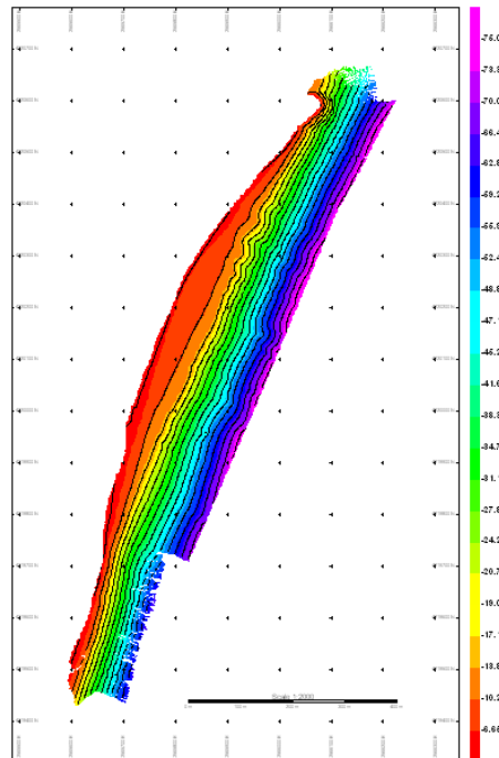
2D BATHYMETRIC PLAN
