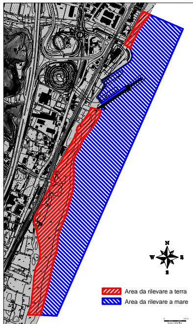
BATHYMETRIC AND TOPOGRAPHICAL SURVEY AREA
