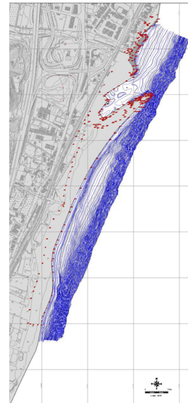
ISOBATH LINES AND TOPOGRAPHICAL HEIGHTS
