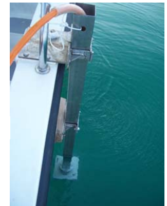
SUBBOTTOM EQUIPMENT
