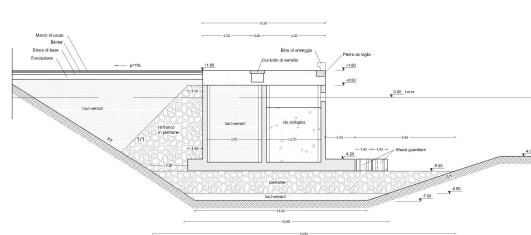
SEA WORKS TYPE SECTIONS
