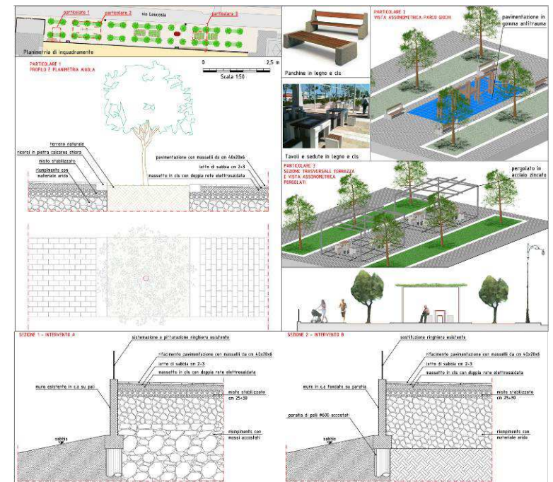
DETAILS OF LAND WORKS
