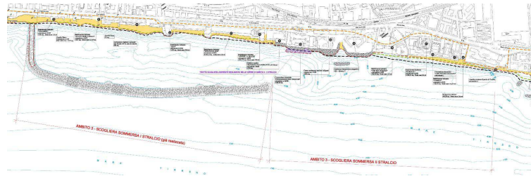
CURRENT LAYOUT
