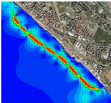
HYDRODYNAMIC STUDIES
